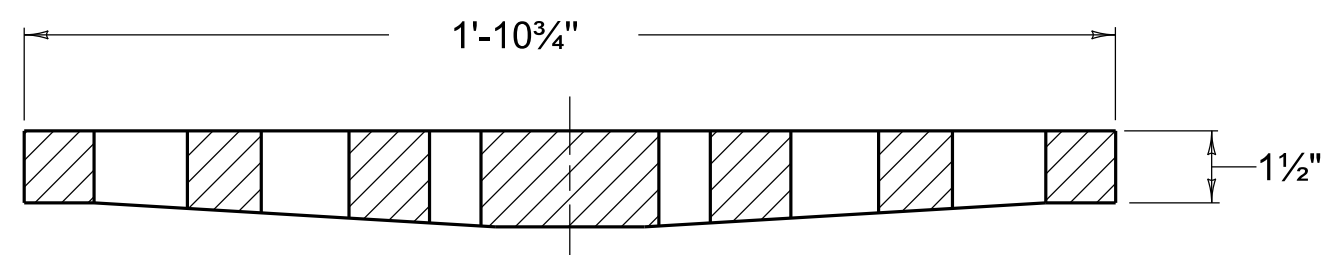
SECTION B-B TYPE 14 (RADIAL)
