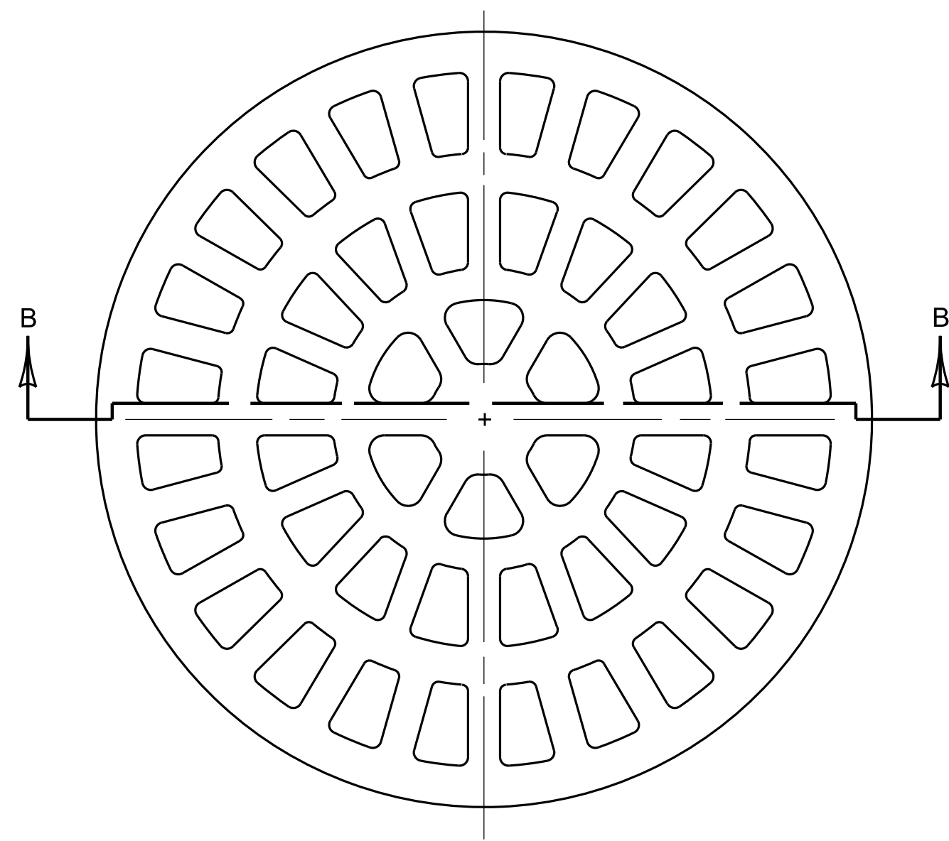
PLAN VIEW
